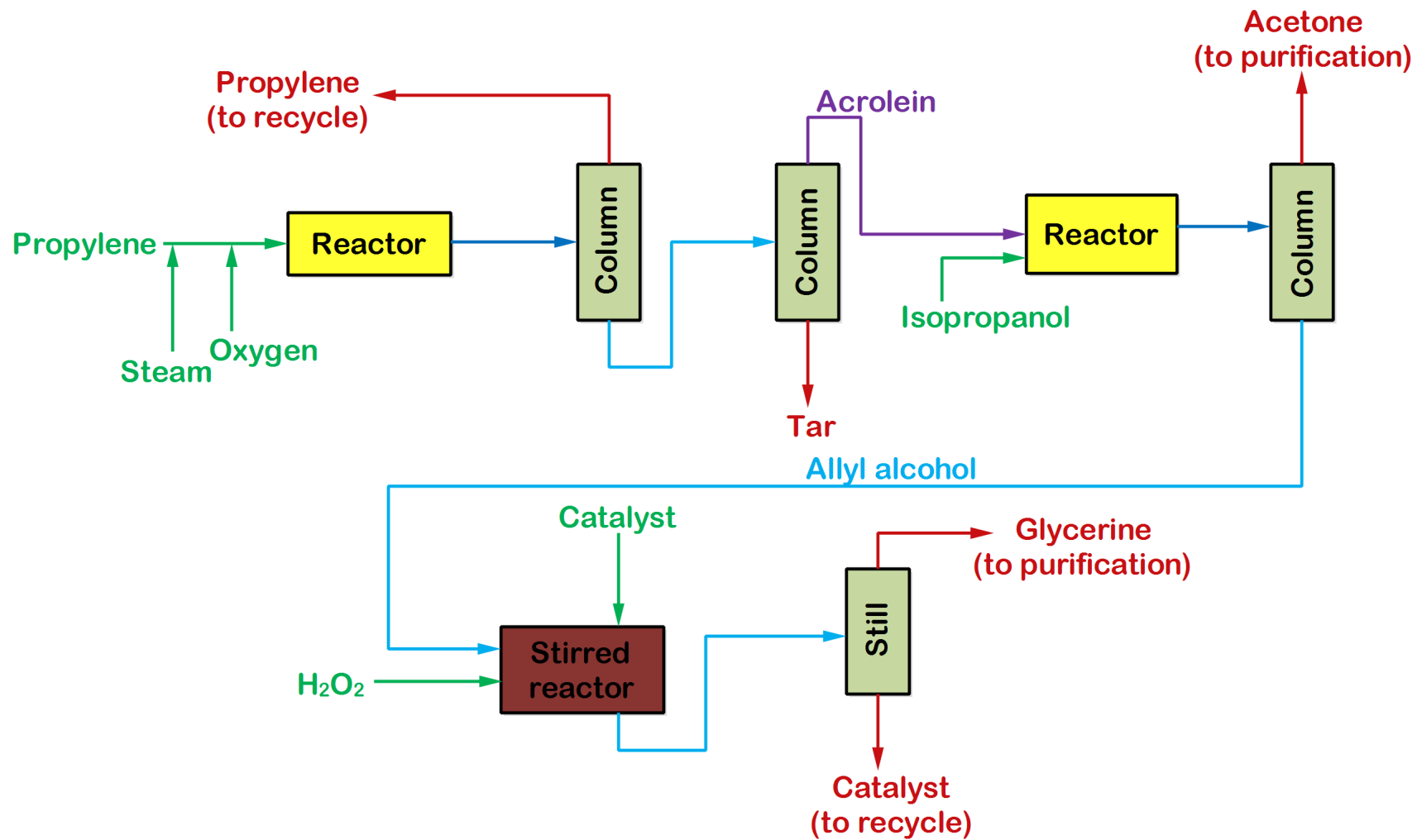
Figure: Manufacture of Glycerol from propylene via acrolein
